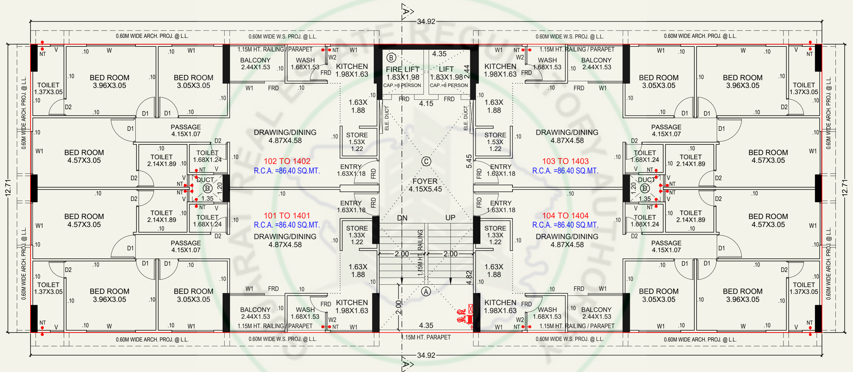
1ST TO 14TH FLOOR PLAN (BLOCK-B)
