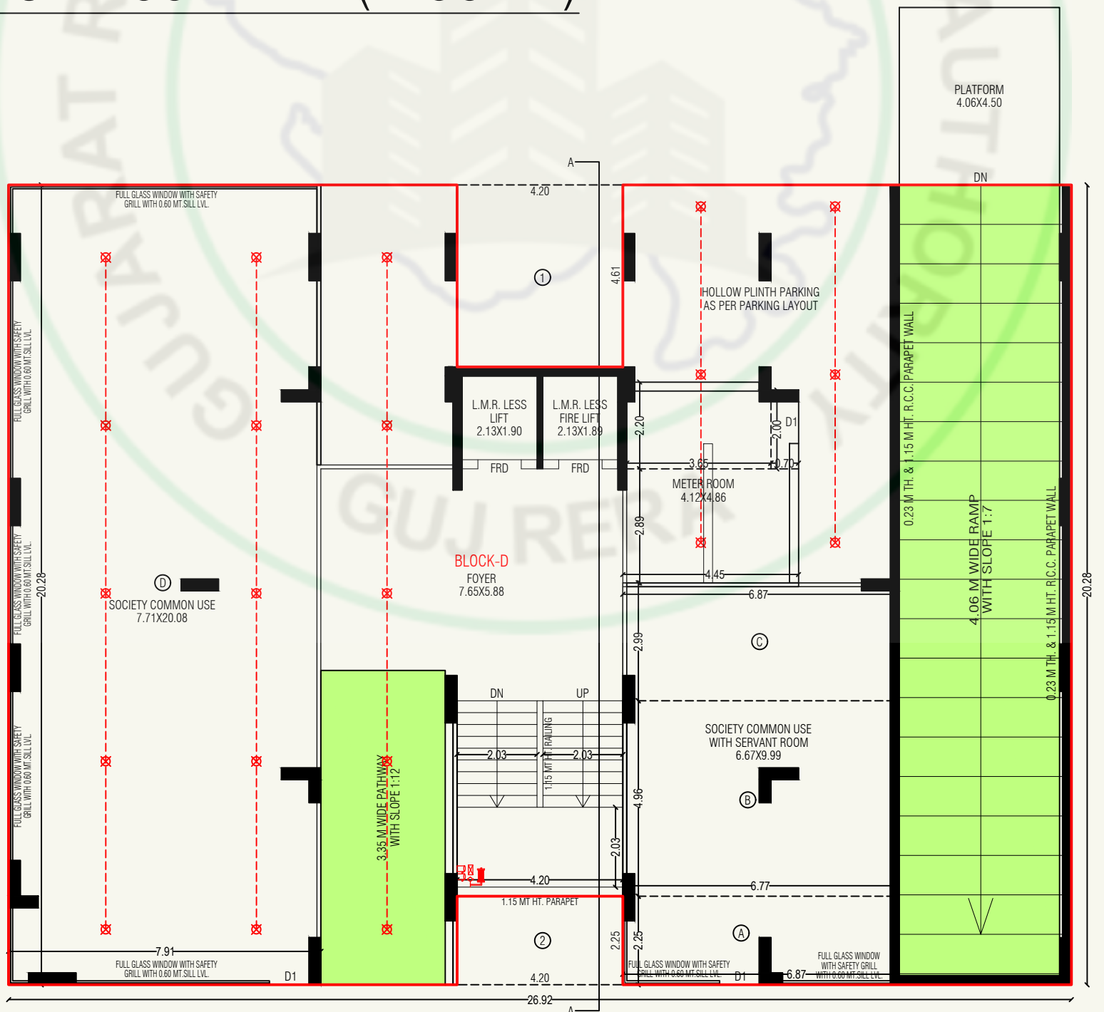
GROUND FLOOR PLAN (BLOCK-D)
