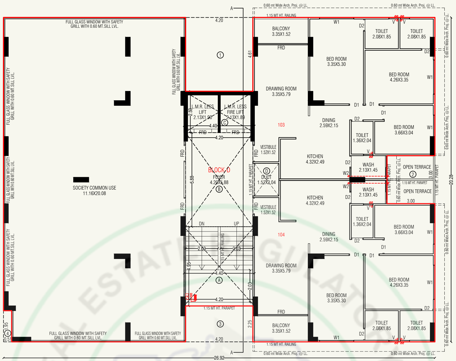
1ST FLOOR PLAN (BLOCK-D)
