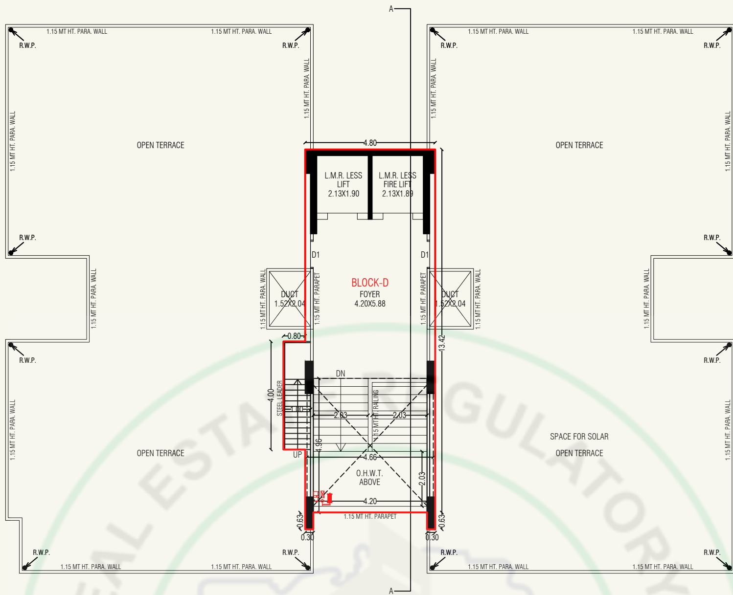
STAIR CABIN/TERRACE PLAN (BLOCK-D)
