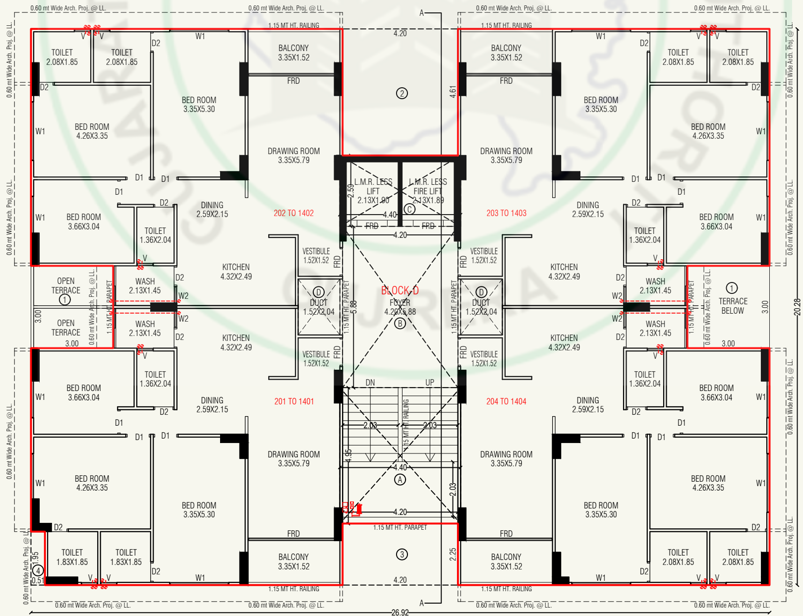
2ND TO 14TH FLOOR PLAN (BLOCK-D)
